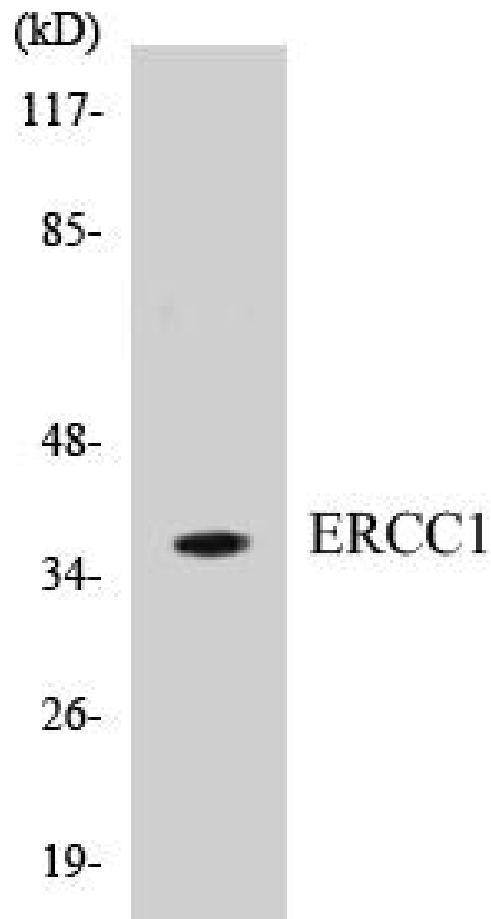
Figure 2. Western blot analysis of the lysates from HeLa cells using ERCC1 antibody.
