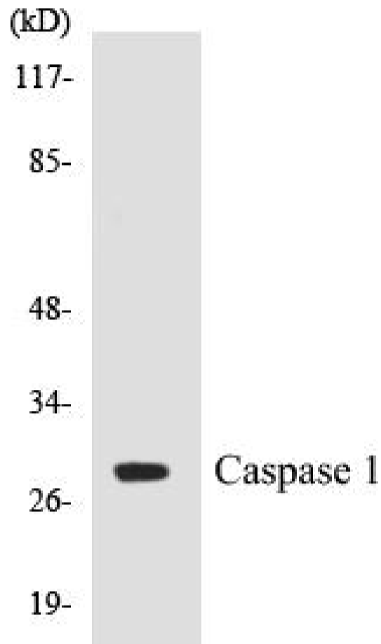
Figure 2. Western blot analysis of extracts from 293/MCF-7/HeLa cells, using Caspase 1 (Ab-376) Antibody.
