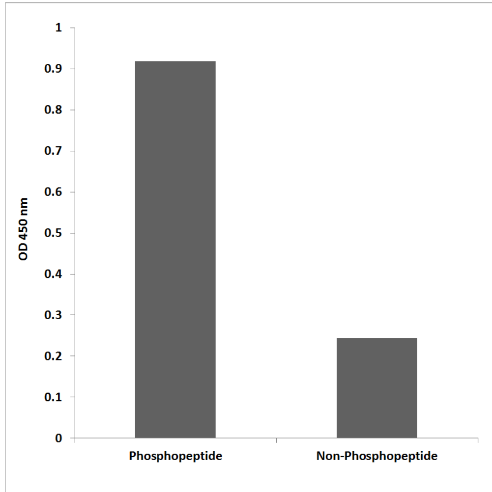
Figure 3. Enzyme-Linked Immunosorbent Assay (ELISA) for immunogen phosphor-peptide (left) and non-phospho peptide (right), using Anti-STAT3 (Phospho-Ser727) Antibody.
