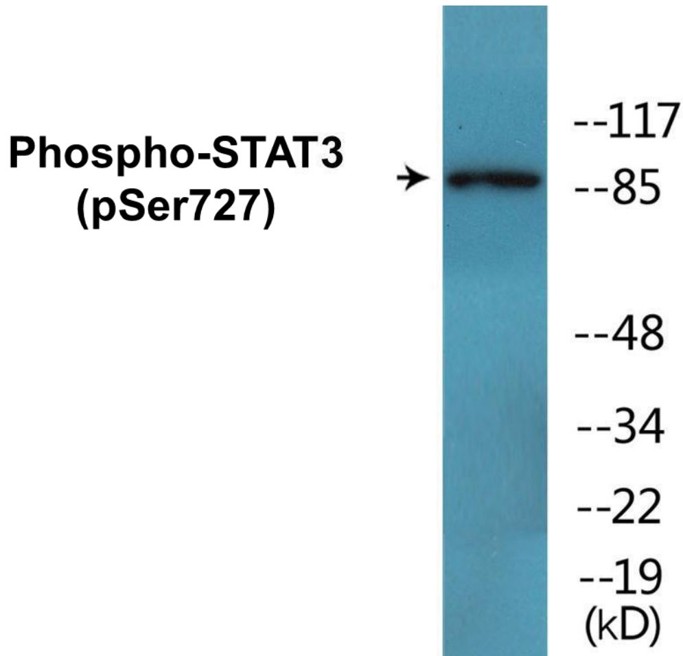
Figure 2. Western blot analysis of extracts from COS7 cells using the Anti-STAT3 (Phospho-Ser727) Antibody.
