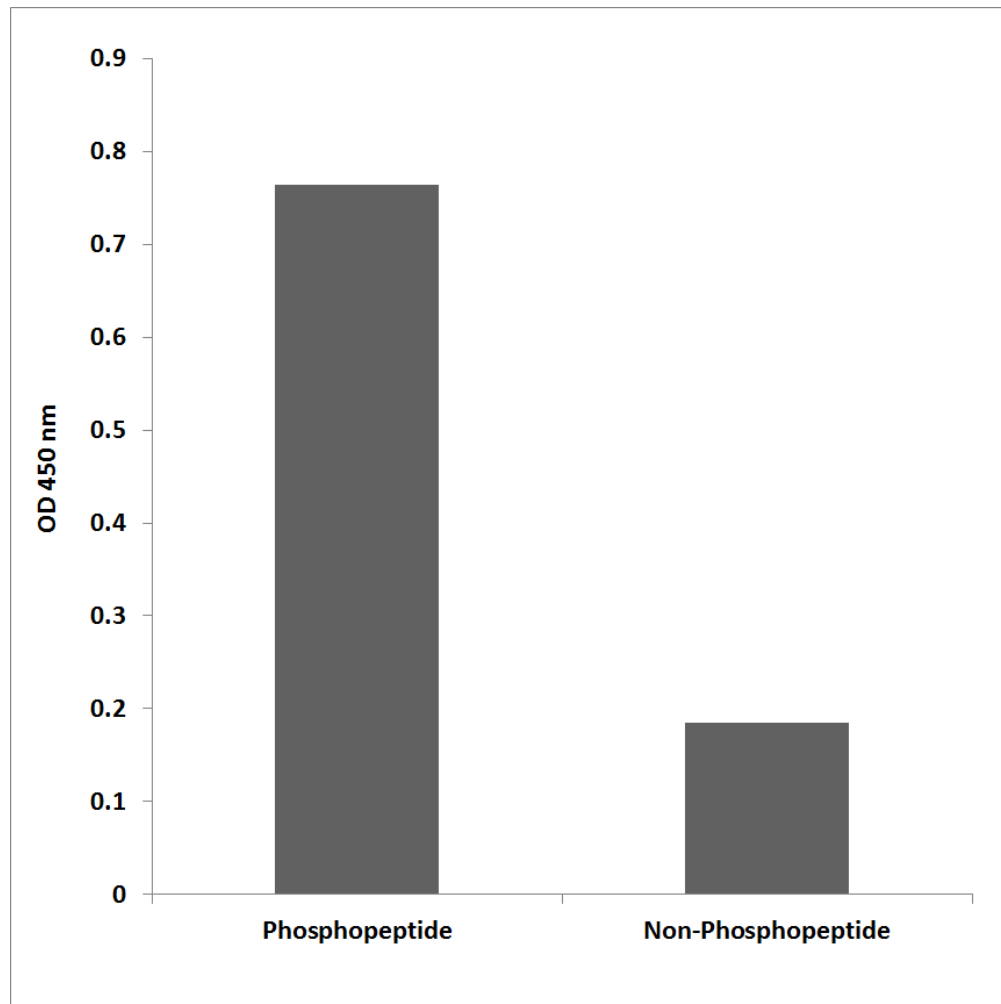
Figure 3. Enzyme-Linked Immunosorbent Assay (ELISA) for immunogen phosphor-peptide (left) and non-phospho peptide (right), using Anti-PDK1 (Phospho-Ser241) Antibody.
