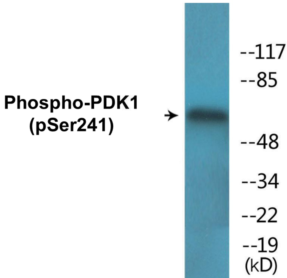
Figure 2. Western blot analysis of extracts from HeLa cells and NIH/3T3 cells, using the Anti-PDK1 (Phospho-Ser241) Antibody.
