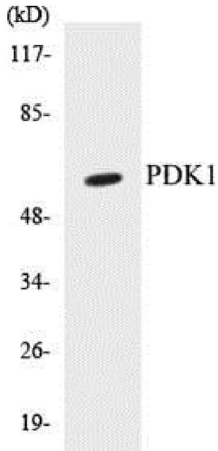
Figure 4. Western blot analysis of extracts from MDA-MB-435 cells, treated with EGF, using the Anti-PDK1 Antibody.
